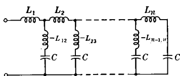
FIG. 6-20.—Pulse-forming network having equal capacitances.
